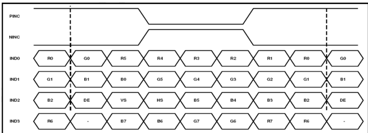
Fig6: LVDS Data Mapping
